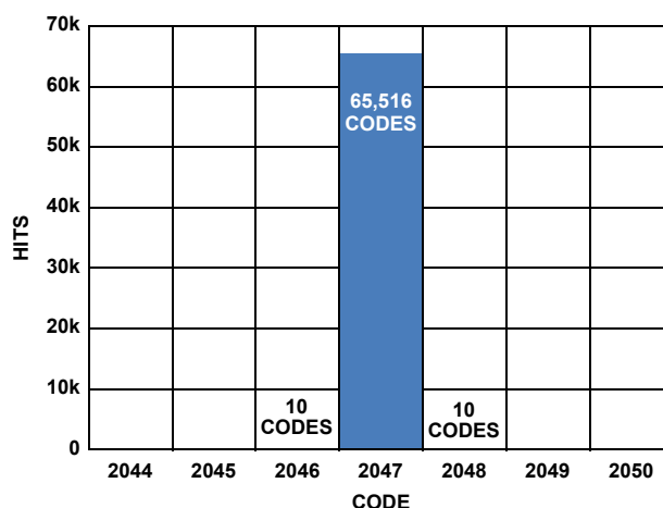
FIGURE 18. HISTOGRAM OF 10,000 CONVERSIONS OF A DC INPUT FOR THE ISL267452 WITH VDD = 5V
