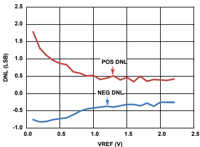
FIGURE 14. CHANGE IN DNL vs VREF FOR THE ISL267452 FOR VDD = 3V
