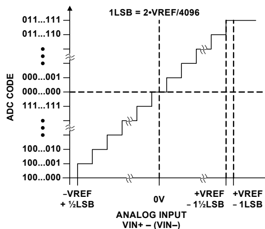
FIGURE 20. IDEAL TRANSFER CHARACTERISTICS
