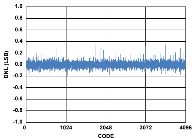
FIGURE 9. TYPICAL DNL FOR THE ISL267452 FOR VDD = 5V
