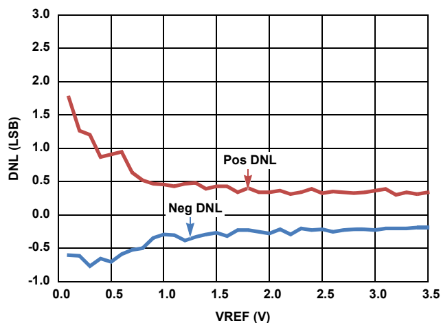
FIGURE 12. CHANGE IN DNL vs VREF FOR THE ISL267452 FOR VDD = 5V
