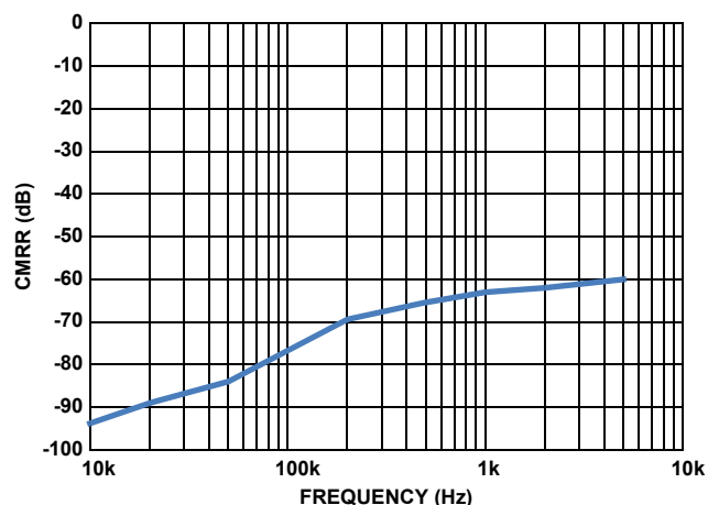
FIGURE 8. CMRR vs FREQUENCY FOR VDD = 5V
