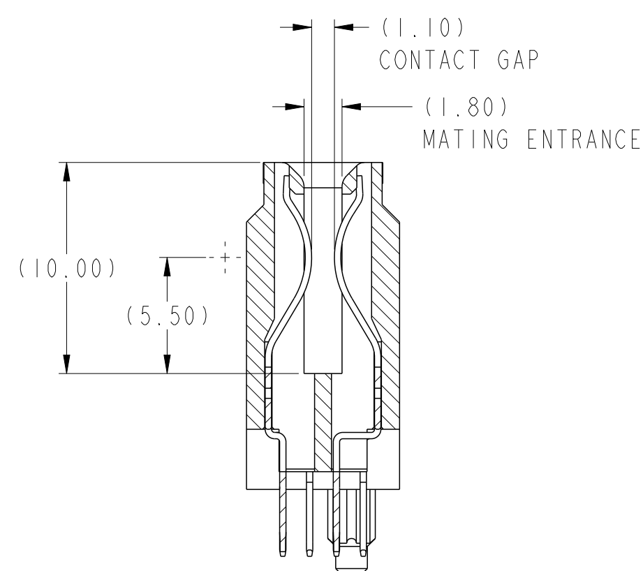
SECTION B-B
