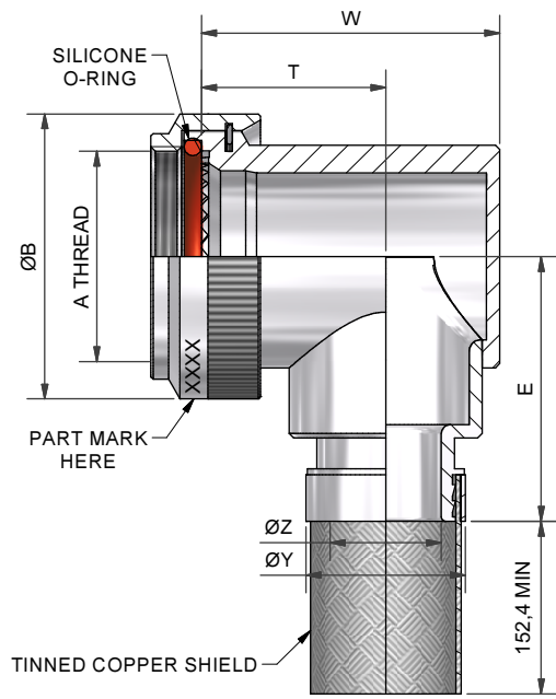
90° BACKSHELL - TYPE 1
