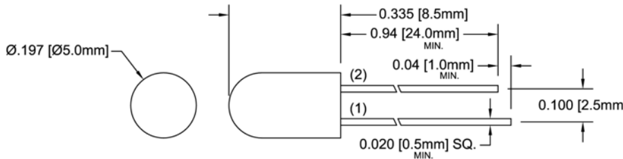
Standard "5BC" LED
