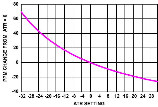
FIGURE 10. ΔF OUT vs ATR SETTING
