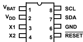
ISL12027, ISL12027A (8 LD TSSOP) TOP VIEW
