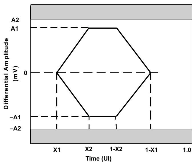
Figure 4-2. Transmit Template
