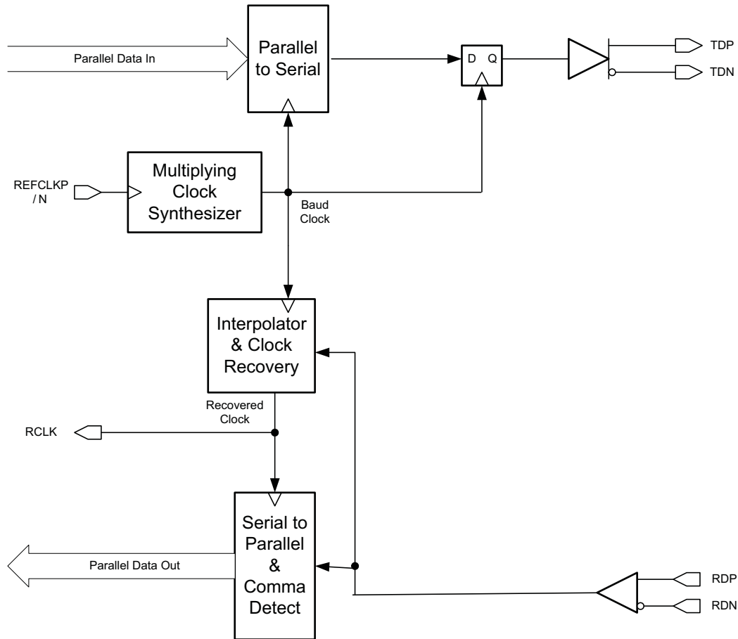
Figure 2-7. Block Diagram of SERDES Core
