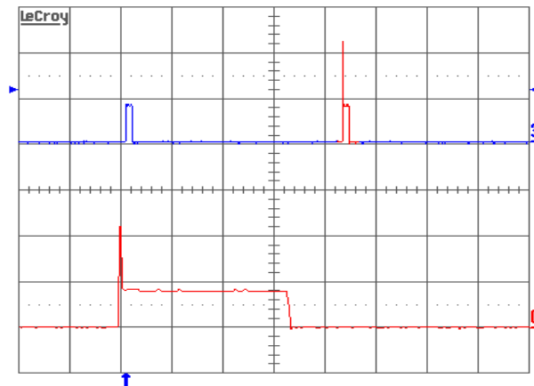
Figure 14. Load current (top trace, 5 A/div., 50 ms/div.) into a 10\ \text{m}\Omega short circuit during restart, at V_{in} = 48\ \text{V} . Bottom trace (5 A/div., 2 ms/div.) is an expansion of the on-time portion of the top trace.
