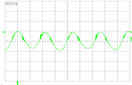
Figure 13. Input reflected ripple-current, i_c (50 mA/div.), measured at input terminals at full rated load current and V_{in} = 48\ \text{V} . Refer to Figure 11 for test setup. Time scale: 1\ \mu\text{s}/\text{div} .
