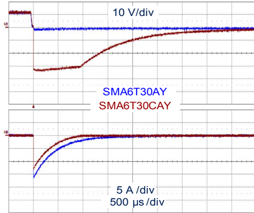
Figure 12. ISO7637-2 pulse 1: V_s = -150\text{ V} with 12 V battery
