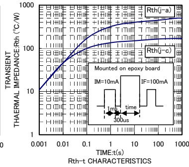
Rth-t CHARACTERISTICS
