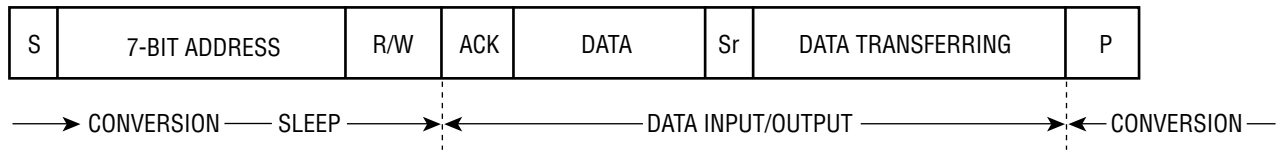
Figure 6. Conversion Sequence
