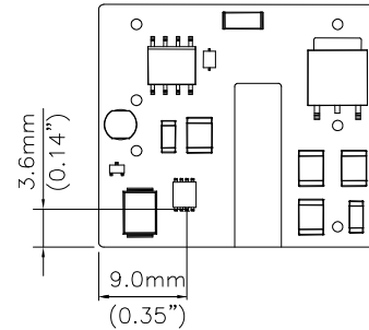
Figure 20: Temperature measurement location
