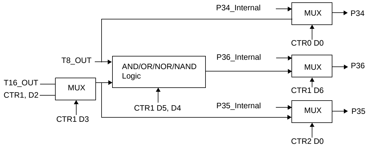
Figure 24. Output Circuit
