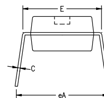
Figure 55. 20-Pin DIP Package Diagram
