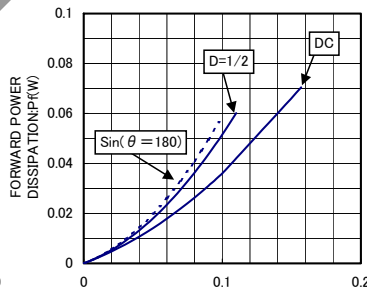
Io-PF CHARACTERISTICS
