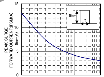
IFSM-t CHARACTERISTICS
