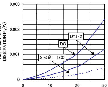
VR-Pr CHARACTERISTICS
