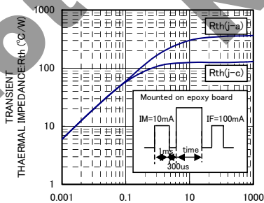
Rth-t CHARACTERISTICS
