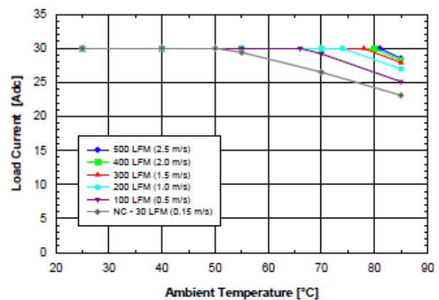
Fig. 1.2V.2: Available load current vs. ambient air temperature and airflow rates for SQE48T30012 converter mounted horizontally with air flowing from pin 3 to pin 1, MOSFET temperature \leq 120^\circ\text{C} , V_{in} = 48\text{ V} .
