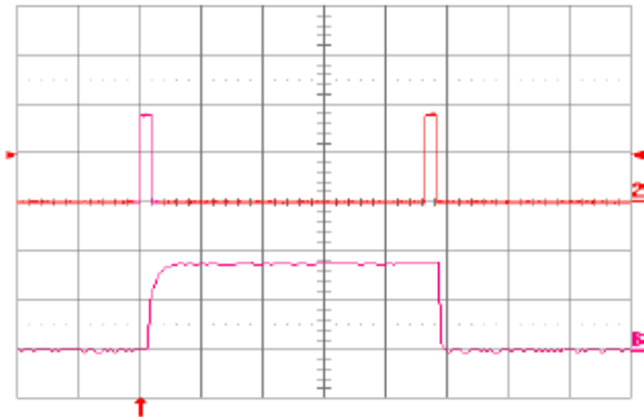
Fig. 1.5V.16: Load current (top trace, 20 A/div., 50 ms/div.) into a 10 mΩ short circuit during restart, at V_{in} = 48\text{ V} . Bottom trace (20 A/div., 2 ms/div.) is an expansion of the on-time portion of the top trace.
