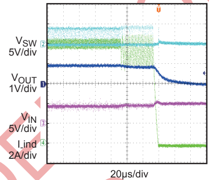
Over-current Protection
