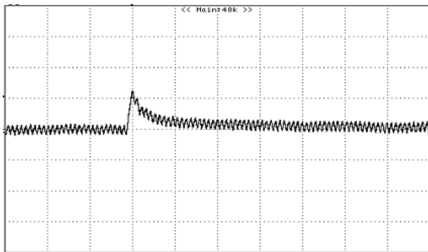
Figure 15: Typical transient response to step load change at 5A/μS from 100% to 50% of I_o , max at 12Vin, 5.0V out ( C_{out} = 1\mu\text{F} ceramic+ 47μF Ceramic)(100mV/div, 20uS/div)
