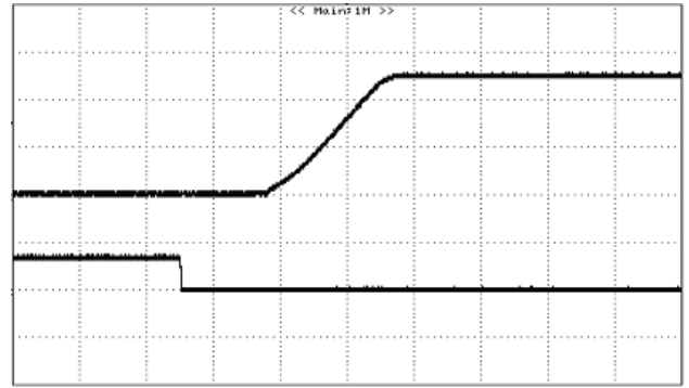
Figure 14: Turn on Using Remote On/Off with external capacitors ( C_o= 3000 \mu\text{F} ), 5.0V/5A out (resistive load)(10mS/div)
