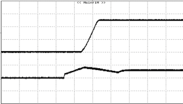
Figure 13: Turn on Using Input On/Off with external capacitors ( C_o=3000 \mu\text{F} ), 5.0V/5A out (resistive load)(10mS/div)
