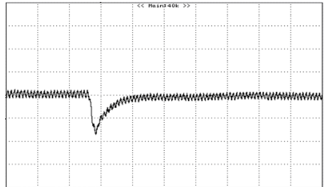
Figure 16: Typical transient response to step load change at 2.5A/μS from 50% to 100% of I_o , max at 12Vin, 5.0V out ( C_{out} = 1\mu\text{F} ceramic+ 10μF Ceramic)(100mV/div, 20uS/div)
