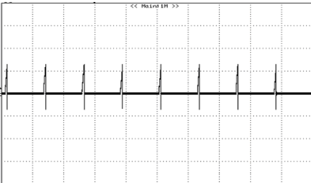
Figure 17: Output short circuit current 12Vin, 0.75Vout (0.5V/div, 50mS/div)
