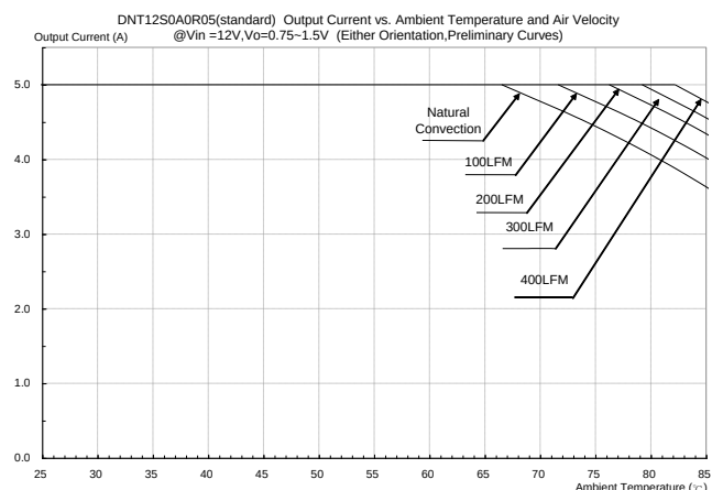
Figure 32: Output current vs. ambient temperature and air velocity@ V_{in}=12V , V_o=0.75-1.5V (Either Orientation, preliminary curves)
