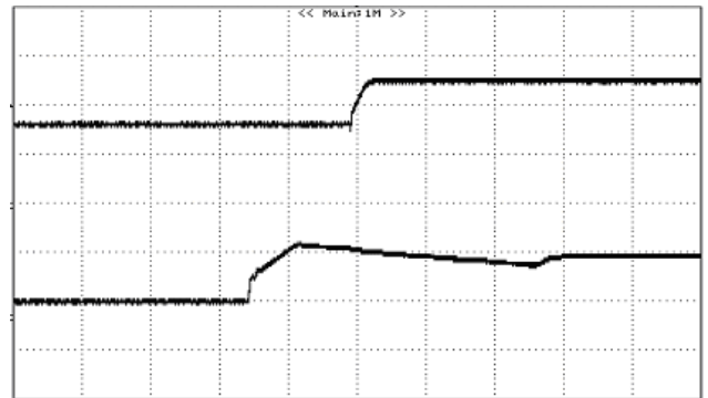
Figure 18: Turn on with Prebias 12Vin, 5V/0A out, V_{bias} = 3.3\text{Vdc} . (5mS/div)
