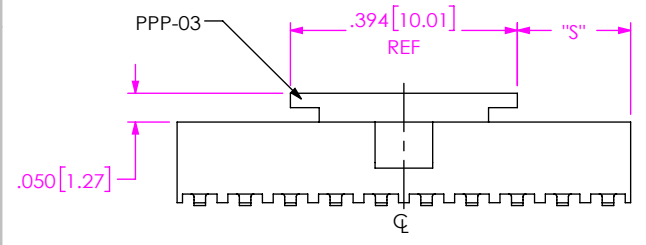
FIG 3 -P: PICK AND PLACE PAD (PLACE PPP-03 ABOUT CL AS SHOWN) (SAME AS FIG 1, DIFFERENT AS SHOWN) (SEE NOTE 9)
