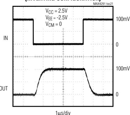
SMALL-SIGNAL TRANSIENT RESPONSE (INVERTING CONFIGURATION)
