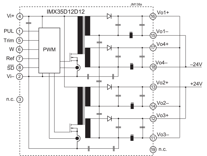
Fig. 7 Generating 24 V with an IMX35D12D12-9
