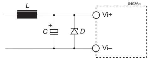
Fig. 4 Example for external circuitry to comply with IEC/EN 61000-4-5; the diode D is only necessary for 20IMX35 models.
