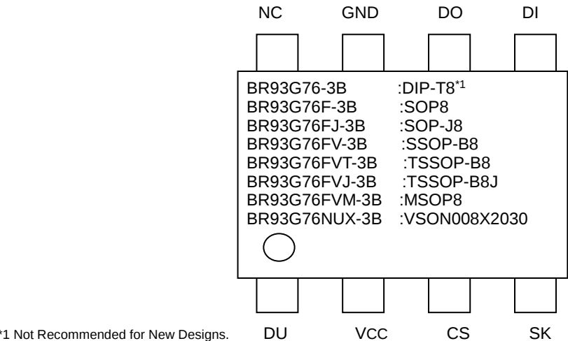
Figure 3. Pin Configuration
