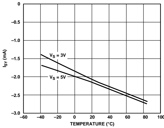
Figure 20. I_{SY-} vs. Temperature
