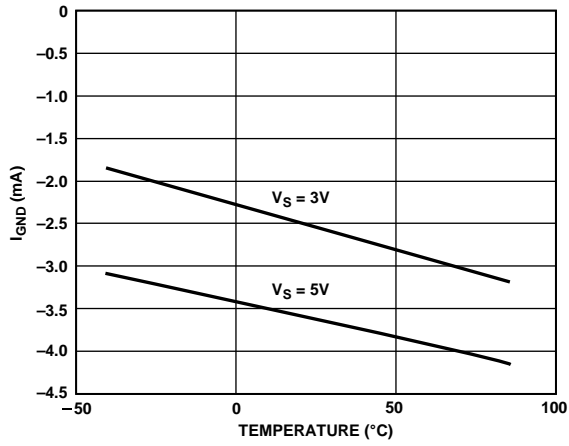
Figure 19. I_{GND} vs. Temperature
