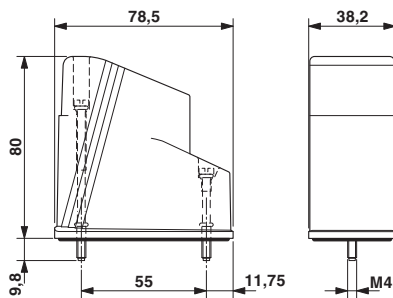
Dimensional drawing
