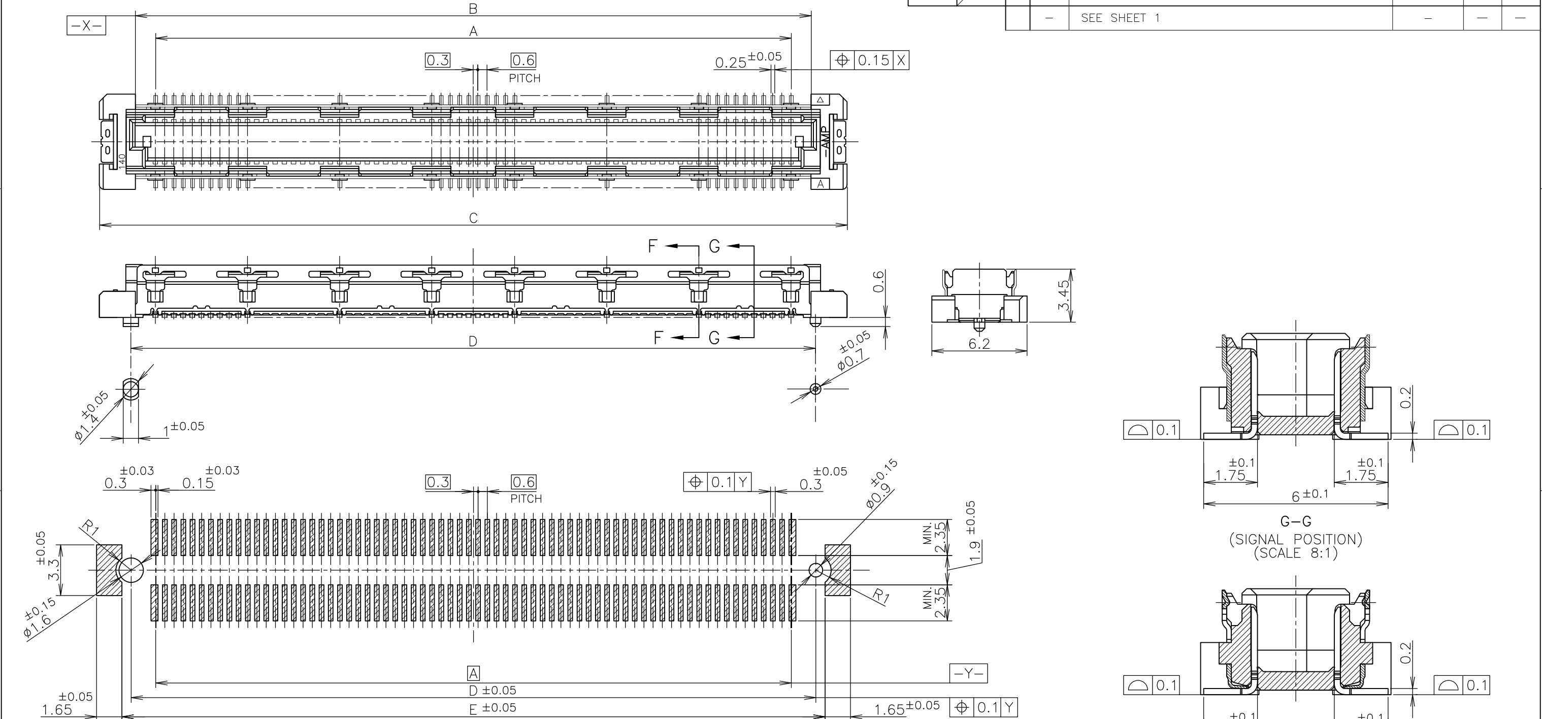
REFERENCE P.C.BOARD LAYOUT
