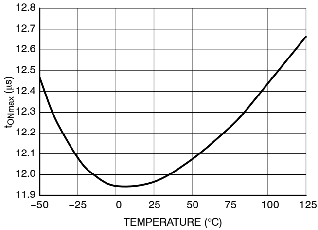
Figure 21. Maximum ON Time t_{ONmax} for the 65 kHz Version
