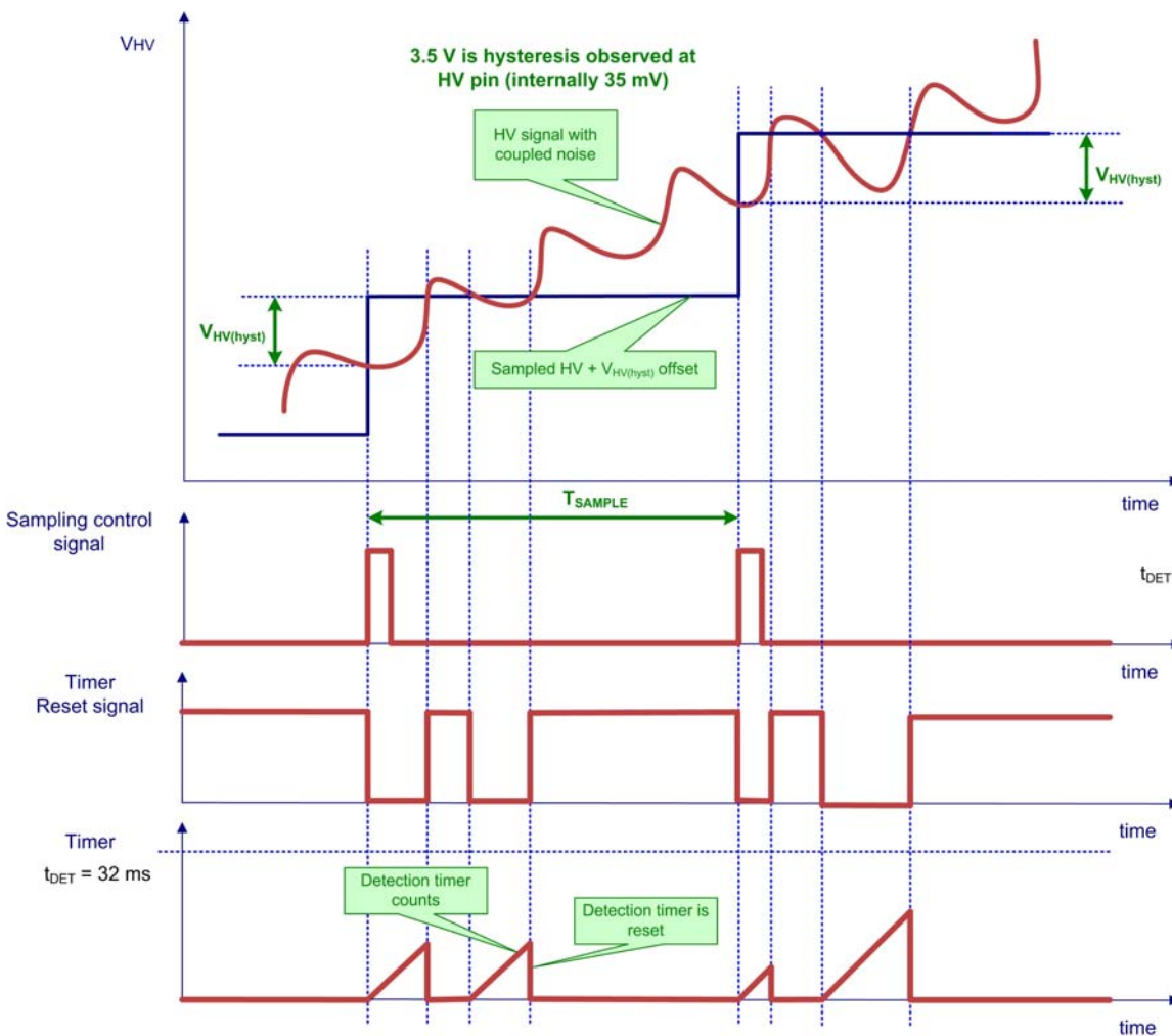
Figure 50. The ac Line Unplug Detector Timing Diagram Detail with Noise Effects
