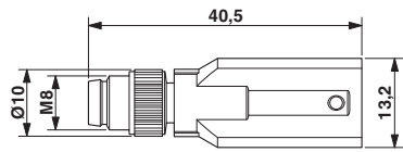
Dimensional drawing
