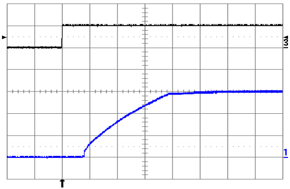
Fig. 6.0V.10: Turn-on transient at full rated load current (resistive) plus 10,000 µF at V_{in} = 24\text{V} , triggered via ON/OFF pin. Top trace: ON/OFF signal (5 V/div.). Bottom trace: output voltage (2 V/div.). Time scale: 2 ms/div.
