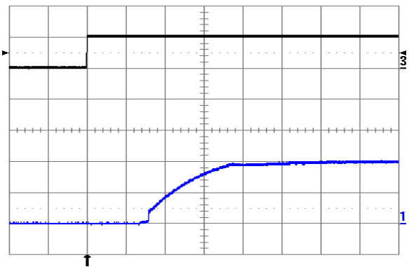
Fig. 2.0V.10: Turn-on transient at full rated load current (resistive) plus 10,000 µF at V_{in} = 24\text{V} , triggered via ON/OFF pin. Top trace: ON/OFF signal (5 V/div.). Bottom trace: output voltage (1 V/div.). Time scale: 1 ms/div.
