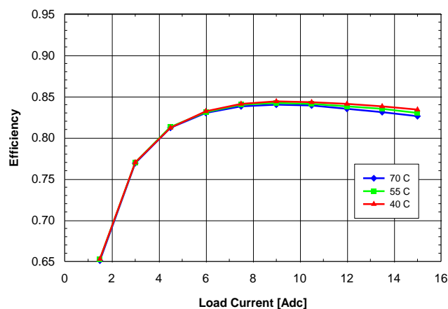
Fig. 1.5V.6: Efficiency vs. load current and ambient temperature for SQ24T/S15015 converter mounted vertically with V_{in} = 24V and air flowing from pin 3 to pin 1 at a rate of 200 LFM (1.0 m/s).
