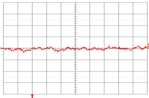
Fig. 3.3V.16: Input reflected ripple current, i_s (10 mA/div.), measured through 10\ \mu\text{H} at the source at full rated load current and V_{in} = 24\ \text{V} . Refer to Fig. 3.3V.14 for test setup. Time scale: 1\ \mu\text{s}/\text{div} .
