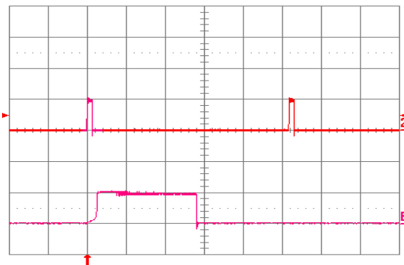
Fig. 3.3V.18: Load current (top trace, 20\ \text{A}/\text{div.} , 20\ \text{ms}/\text{div.} ) into a 10\ \text{m}\Omega short circuit during restart, at V_{in} = 24\ \text{V} . Bottom trace ( 20\ \text{A}/\text{div.} , 1\ \text{ms}/\text{div.} ) is an expansion of the on-time portion of the top trace.
