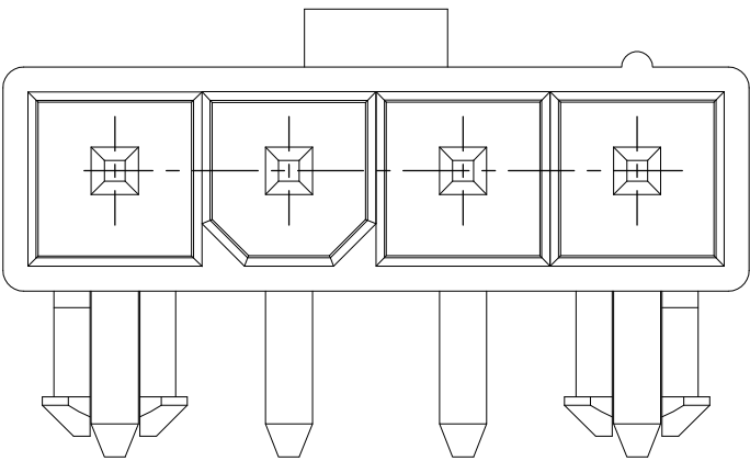
2029151-4 MATING FACE
