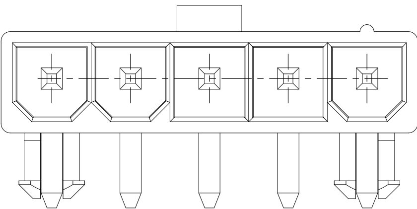
2029151-5 MATING FACE
