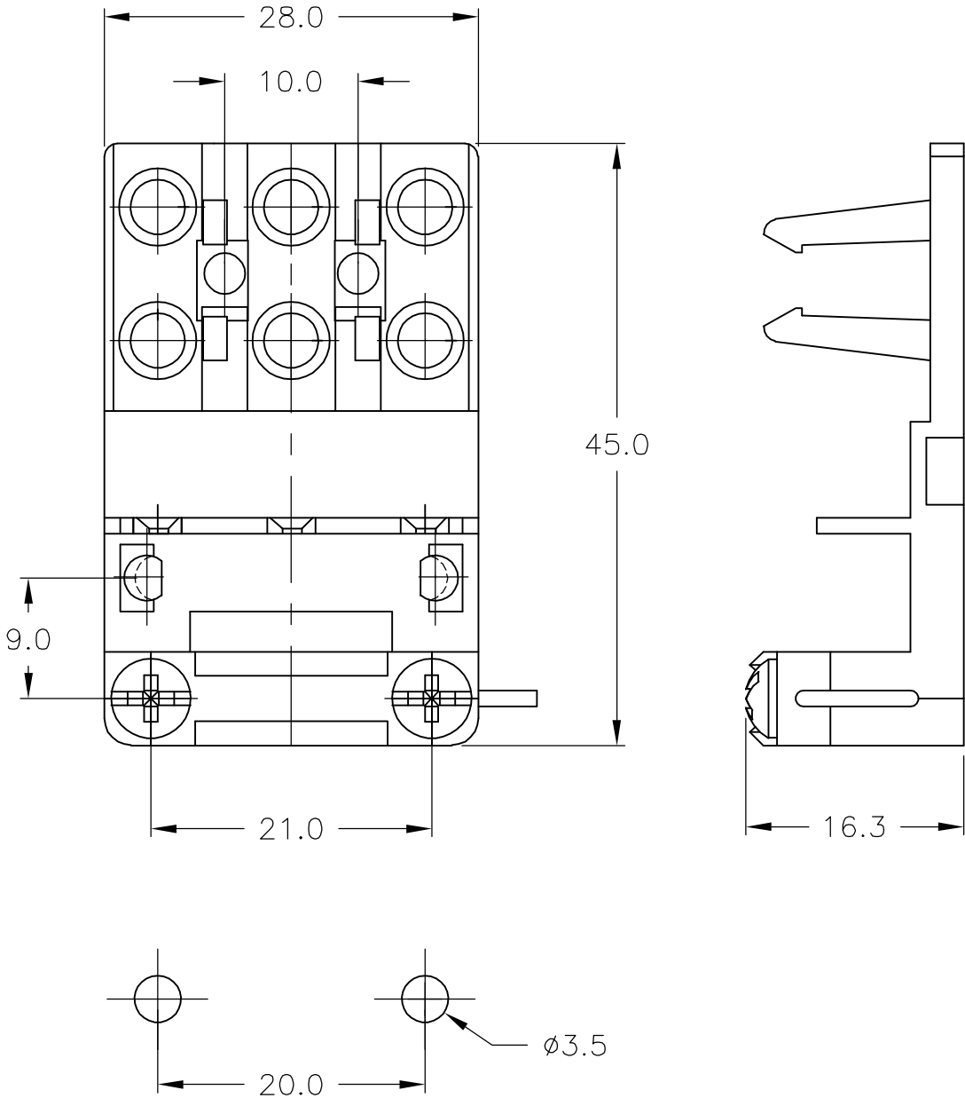
HOLE PATTERN
