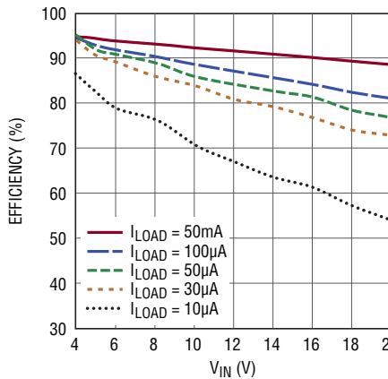
Efficiency vs V_{IN} for V_{OUT} = 3.3\text{V} , L = 100\mu\text{H} (LTC3388-3)
