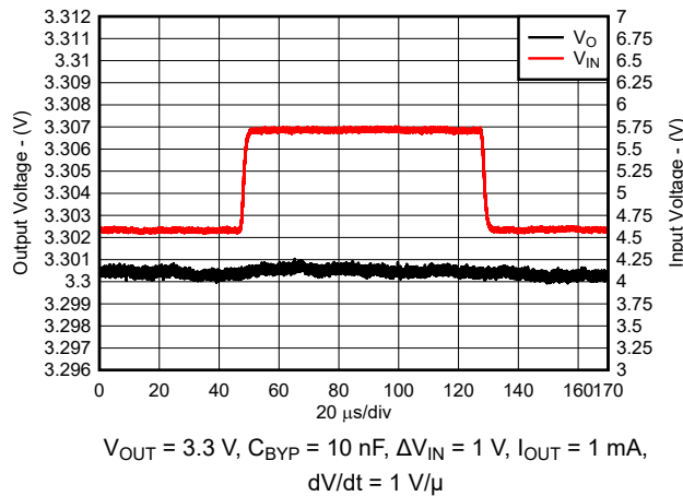
Figure 5-48. Line Transient Response for New Chip
