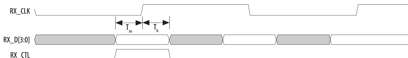
Figure 1-14: RGMII RX Timing Diagram
