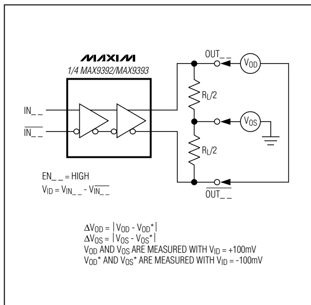
Figure 2. Test Circuit for V_{OD} and V_{OS}
