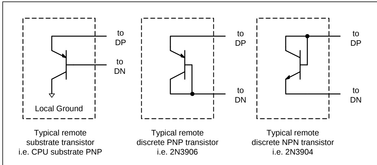
Figure 5.5 Diode Configurations
