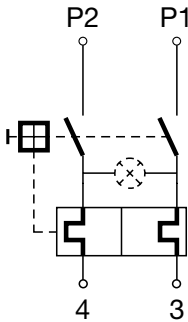
2 pole thermal overload protection
