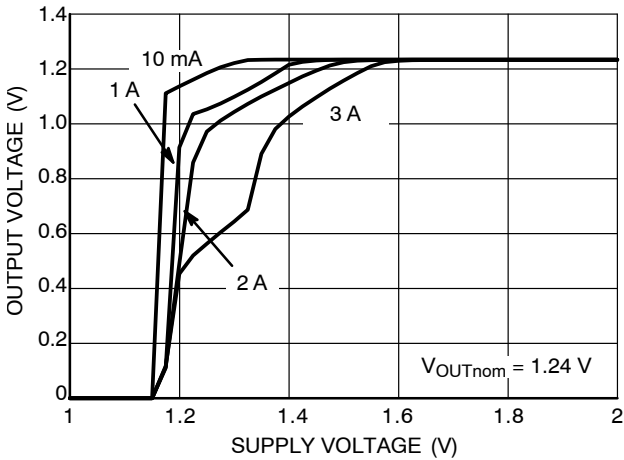
Figure 6. Dropout Characteristics
