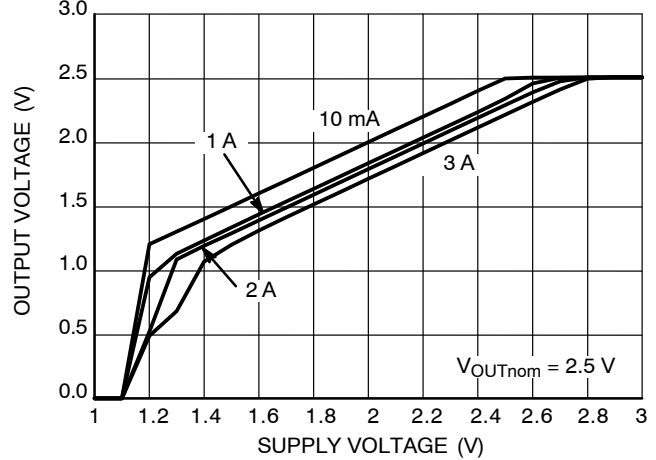
Figure 7. Dropout Characteristics
