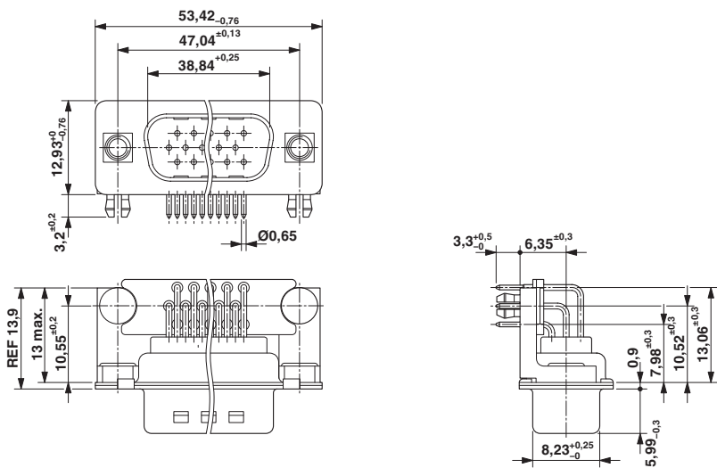
Dimensional drawing
