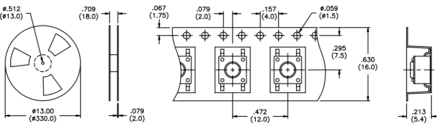
Tape & reel packaging - quantity 1200 per reel.
