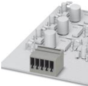
ST-COMBI receptacle, plug-in direction horizontal to the PCB, pitch: 5.2 mm, no. of positions: 10
