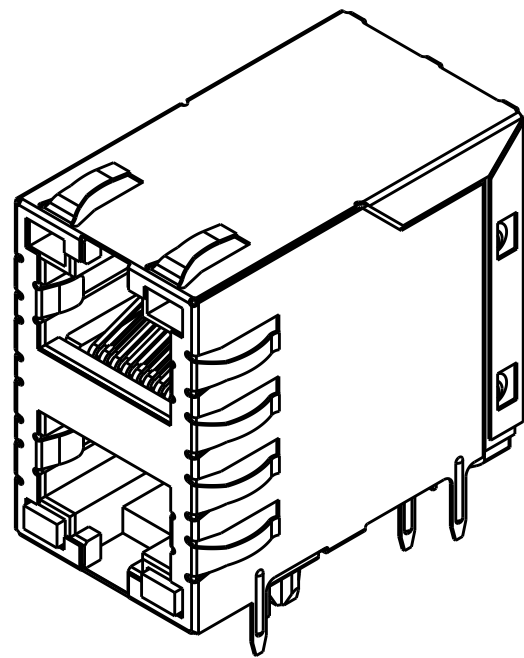
PN 6368011-7 SAME AS 6368011-1 EXCEPT AS SHOWN WITHOUT TOP LED SCALE 2:1
