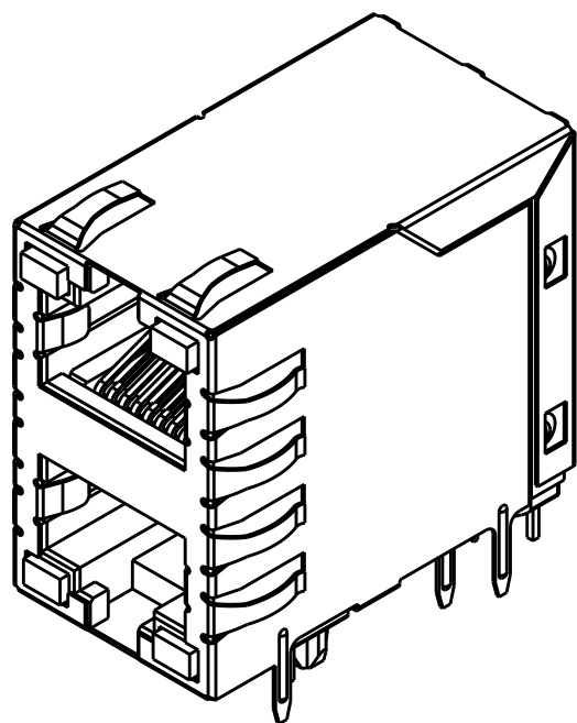
PN 6368011-1,2,3,4,5,6,8 & 1-6368011-0,1,5 SCALE 2:1
