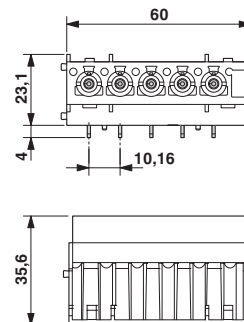
Dimensional drawing
