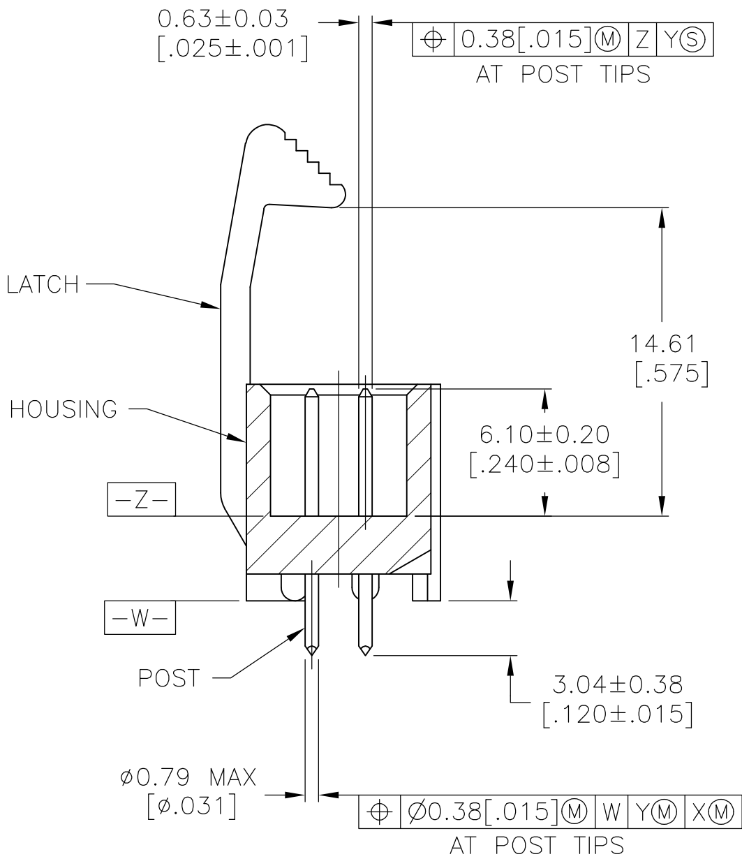
SECTION U-U
