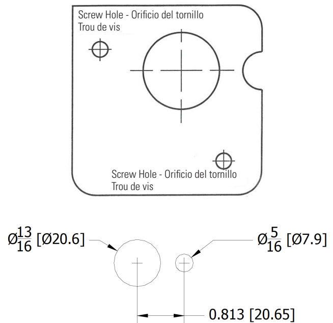
Figure 2: Mounting Template
