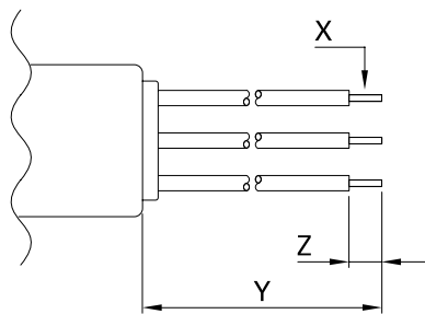
-07 connection style
