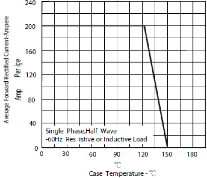
Figure.2-Forward Derating Curve
