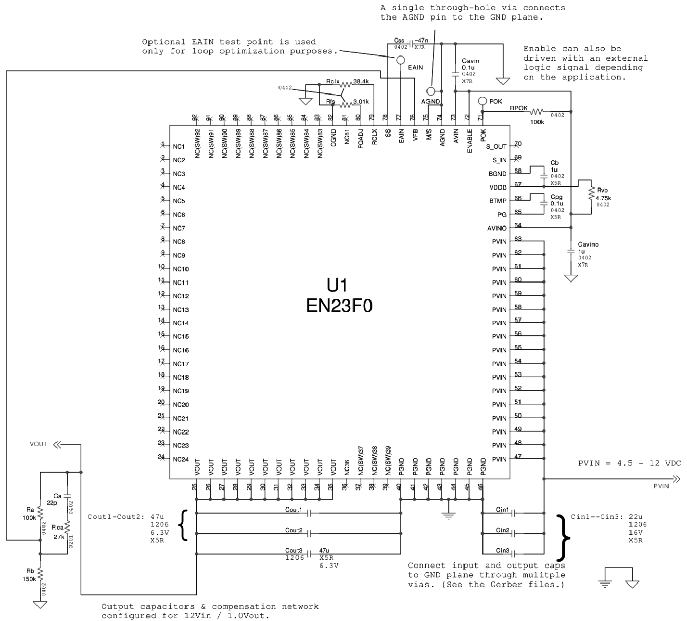
Figure 12: Critical Components Engineering Schematic
