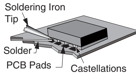
Figure 35: Soldering Technique
