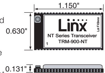
Figure 1: Package Dimensions
