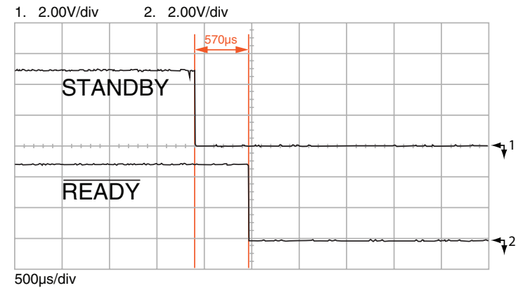
Figure 14: NT Series Transceiver Turn-On Time from Standby
