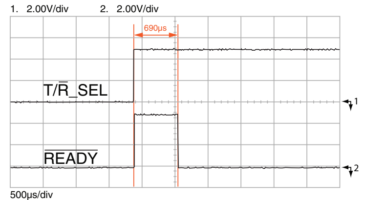
Figure 16: NT Series Transceiver TX to RX Change Time
