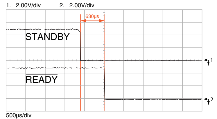
Figure 15: NT Series Transceiver Transmitter Turn-On Time from Standby
