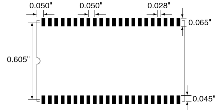
Figure 32: Recommended PCB Layout
