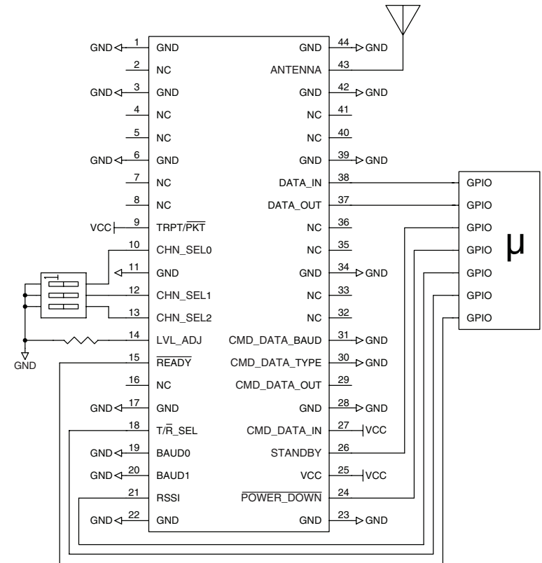
Figure 29: NT Series Transceiver Typical Application
