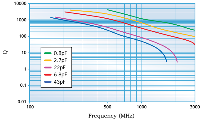
0603 H Series Q vs. Frequency
