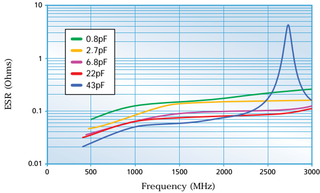
0603 H Series ESR vs. Frequency
