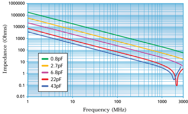
0603 H Series Impedance vs. Frequency
