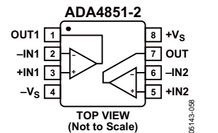
图2. ADA4851-2 8引脚MSOP (RM-8)
