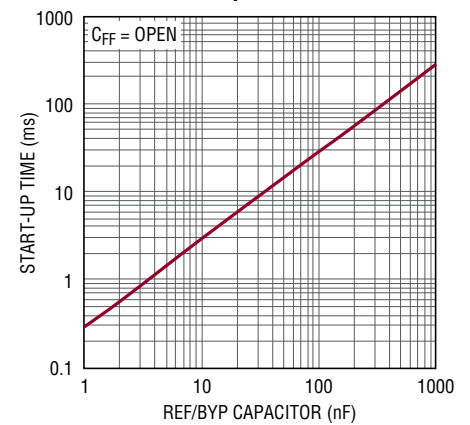
Start-Up Time vs REF/BYP Capacitor
