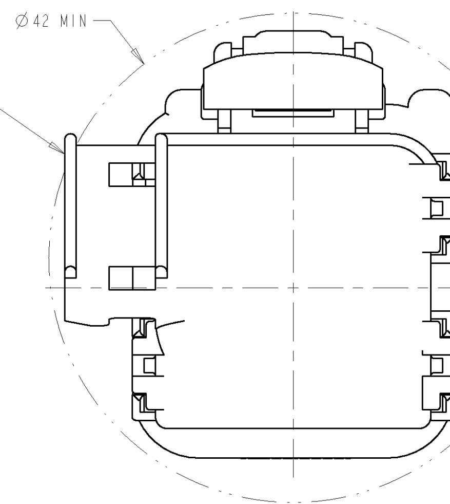
MINIMUM FEED THROUGH CONDITION WITH 1mm CLEARANCE ALL AROUND SHOWN WITH OPTION WIRESHIELD
